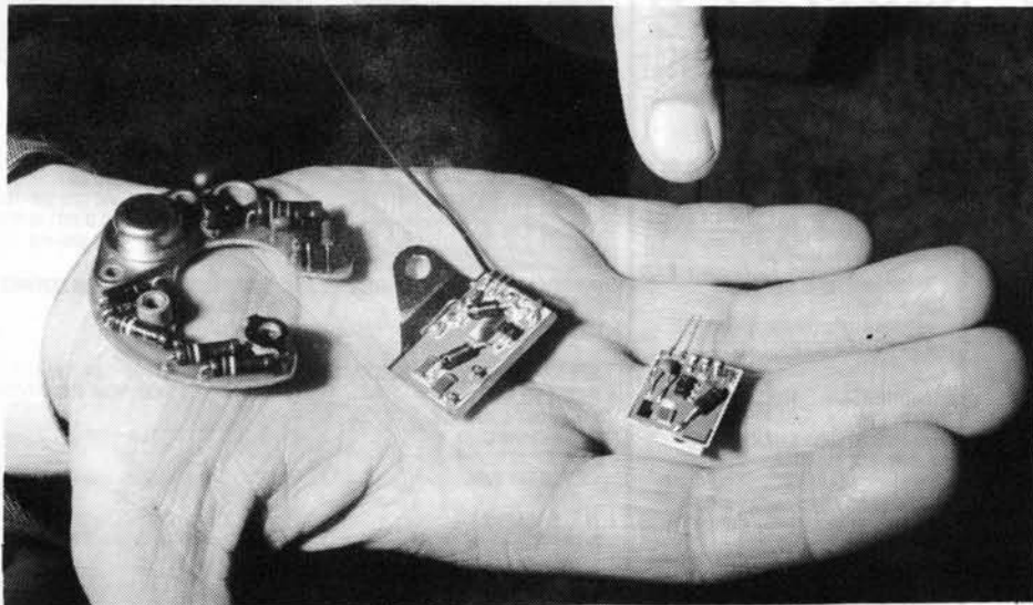
Three stages in the development of transistorized ignition systems for Stihl Chain Saws - the latest and smallest is on the right.
